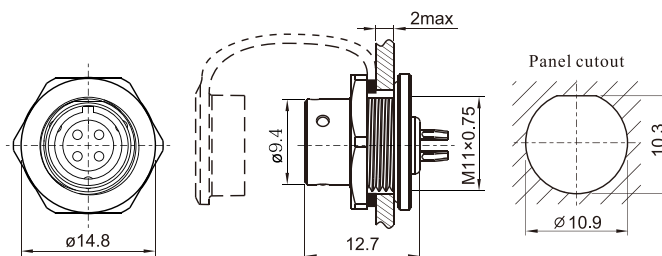
Front-nut mount Mate with SF810B
