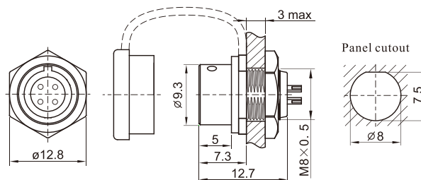
Rear-nut mount Mate with SF810B
