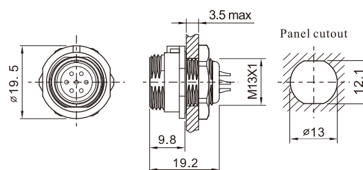
Rear-nut mount Mate with SP1310
