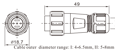
Cable connector Mate with SP1311, SP1312
