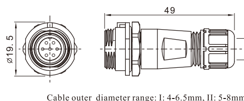
In-line cable connector Mate with SP1310
