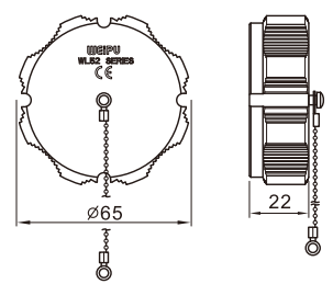
● WL52-GZK IP67 Aluminium cap for female-contact connector
