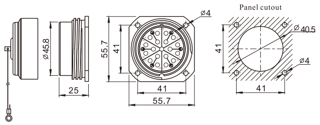
● WL52K19Z IP67 Square flange female contact receptacle
