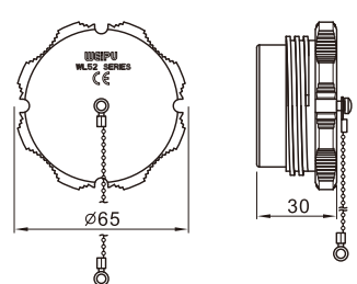
● WL52-GZJ IP67 Aluminium cap for male-contact connector
