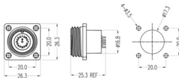
S socket (dimensions figure)
