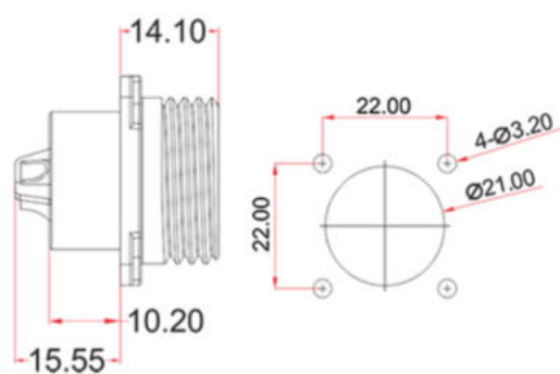
Installation hole figure
