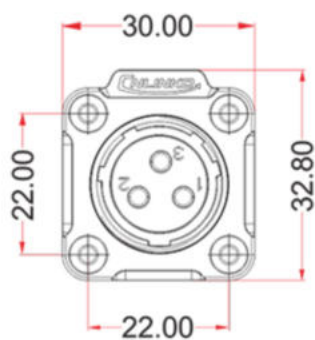
S socket (dimensions figure)
