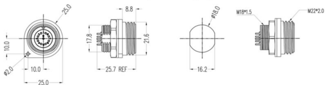
S socket (dimensions figure)
