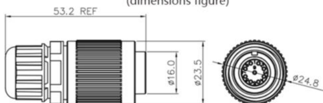
PE clamping cable plug (dimensions figure)
